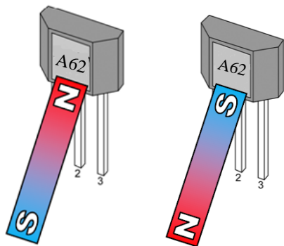
V OUT =低电压 V OUT =高电压 T092S (AH602)
