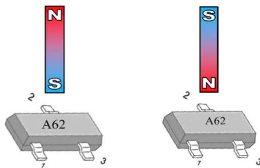
V OUT =低电压 V OUT =高电压 SOT23 (AH602)
